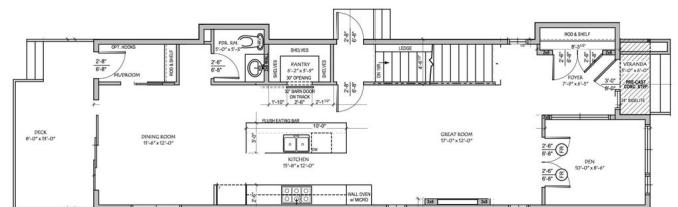
MAIN FLOOR PLAN 946 sq.ft. SCALE: 3/16" = 1'-0"
